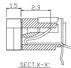
SECT. X-X'
